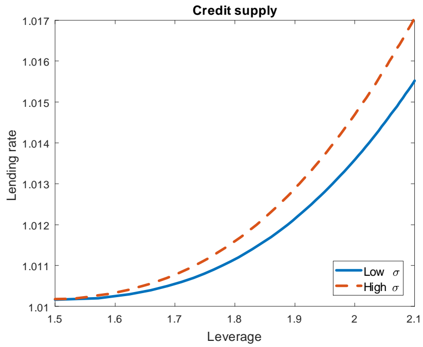
Figure 3. Volatility and credit supply. This figure plots the leverage ratios and gross lending rates that satisfy the lenders' participation constraint (20) for a high ( -2.5 ) and a low ( -4.57 ) value of the steady state volatility parameter \sigma .
